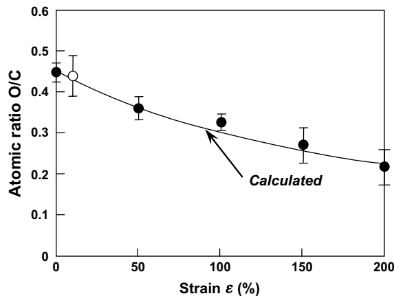
Fig. 3. Effect of strain \epsilon by uniaxial stretching on atomic ratio O/C collected at take-off angle \gamma of 15^\circ of the O_2 -plasma-treated TPFE film. The O/C value of the O_2 -plasma-treated film recovered from 200% stretching was superimposed with open circle. The TPFE film was O_2 -plasma treated at the RF power of 200 W for 60 s.
