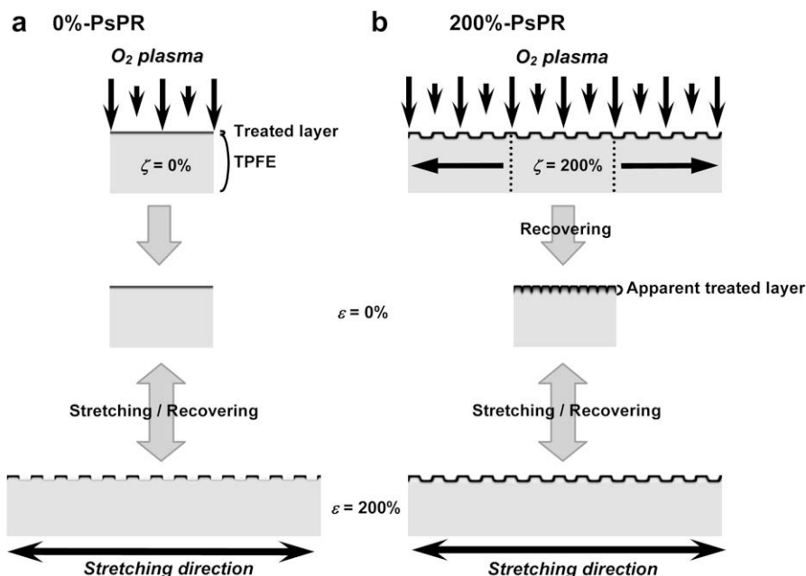
Fig. 8. Schematic illustrations of surface structures of (a) 0%- and (b) 200%-PsPR films before and under uniaxial stretching.
