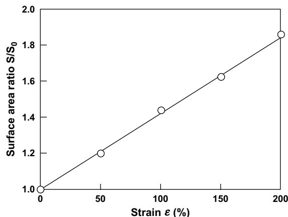
Fig. 2. Relationship between strain \epsilon by uniaxial stretching and macroscopic surface area ratio S/S_0 of the TPFE film. S_0 and S are the surface area before and under uniaxial stretching.
