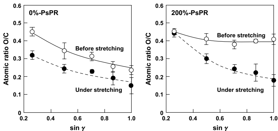
Fig. 7. Angular dependence of atomic ratios O/C for 0%- and 200%-PsPR films before and under uniaxial stretching. The 0%- and the 200%-PsPR films were stretched at \varepsilon = 100\% and \varepsilon = 200\% , respectively. The TPFE films were O_2 -plasma treated at the RF power of 200 W for 60 s.
