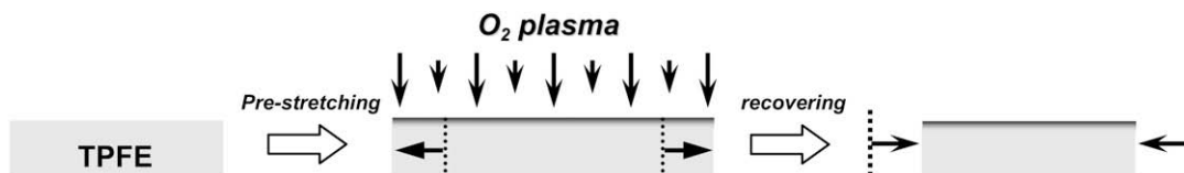
Fig. 5. Schematic illustration of O 2 plasma treatment procedure; Pre-stretching–Plasma treatment–Recovering (PsPR).
