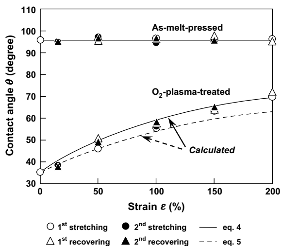
Fig. 1. Effect of strain \epsilon by uniaxial stretching/recovering on contact angle of water for the as-melt-pressed and the O_2 -plasma-treated TPFE film. The TPFE film was O_2 -plasma treated at the RF power of 200 W for 60 s.
