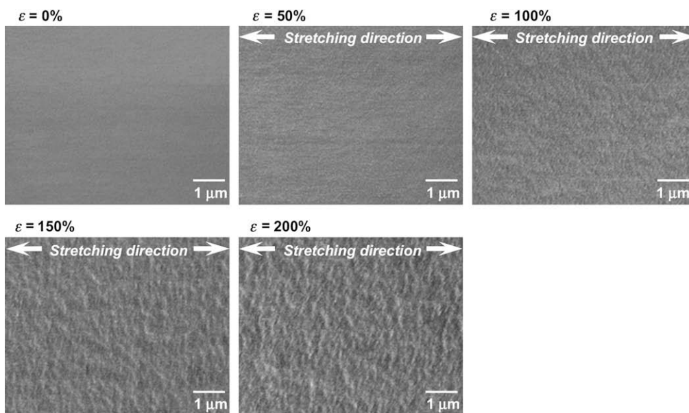
Fig. 4. FE-SEM images of O 2 -plasma-treated TPFE film before and under stretching at \varepsilon = 50\% , 100\% , 150\% and 200\% . The TPFE film was O 2 -plasma treated at the RF power of 200 W for 60 s.
